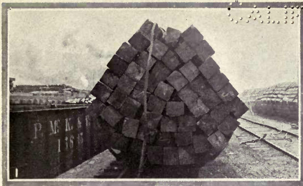
1.—Creosoted ties. Note the S-irons that prevent the spread of checking
